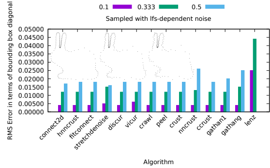
Figure 11: RMS Error of reconstructed curves from ground truth for the sets of cubic Bézier curves in Figure 9, sampled with \epsilon = 0.3 , and the points perturbed with local feature sized noise of \delta = 0.1, \frac{1}{3} and 0.5 (run-lfsnoise.sh). The figure also shows the lfs sampled bunny curve with varying noise (LENZ crashes for \delta = 0.5 , therefore the false 0 value).
